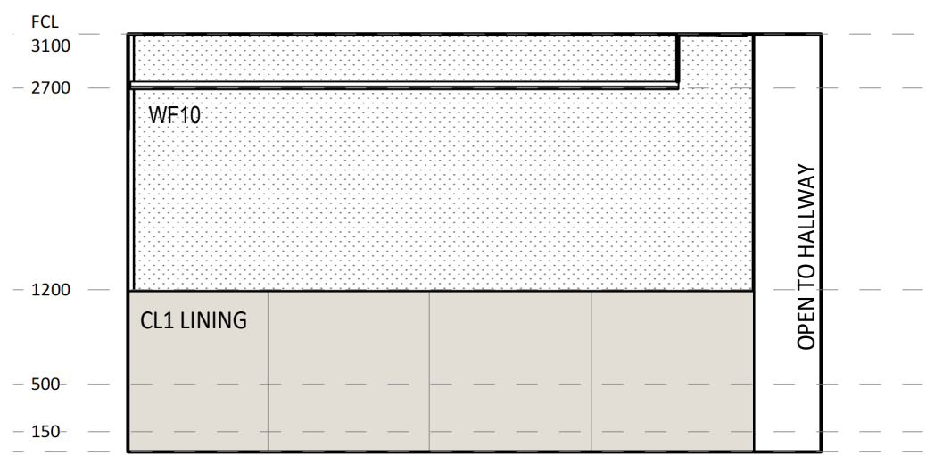
5 ELEVATION DETAIL 60-001 1 : 50
