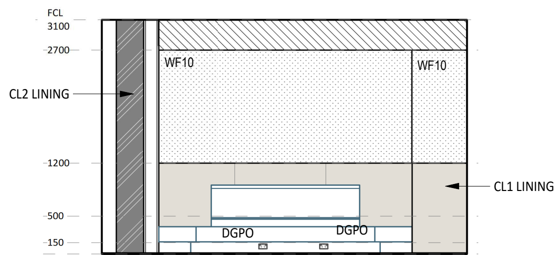
4 ELEVATION DETAIL 60-036 1 : 50
